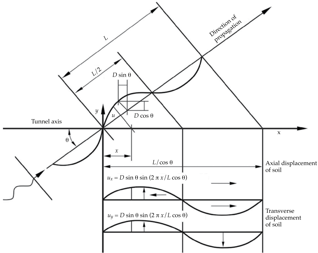
Figure 3. Effect of movement of shear waves along the tunnel axis.
