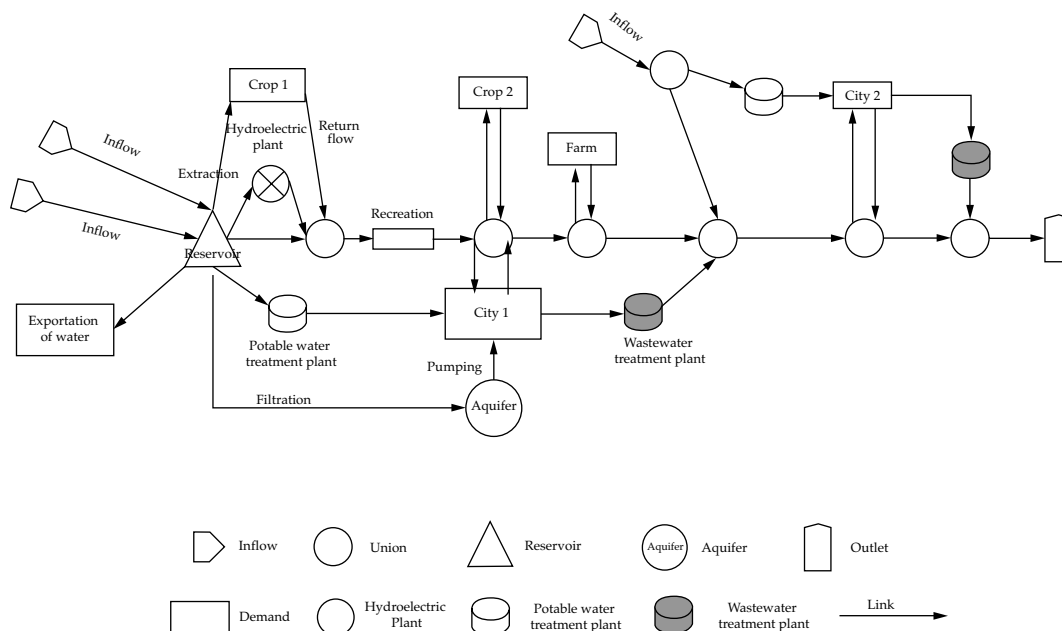
Figure 2. Example of a Hydrographic Watershed Network.
