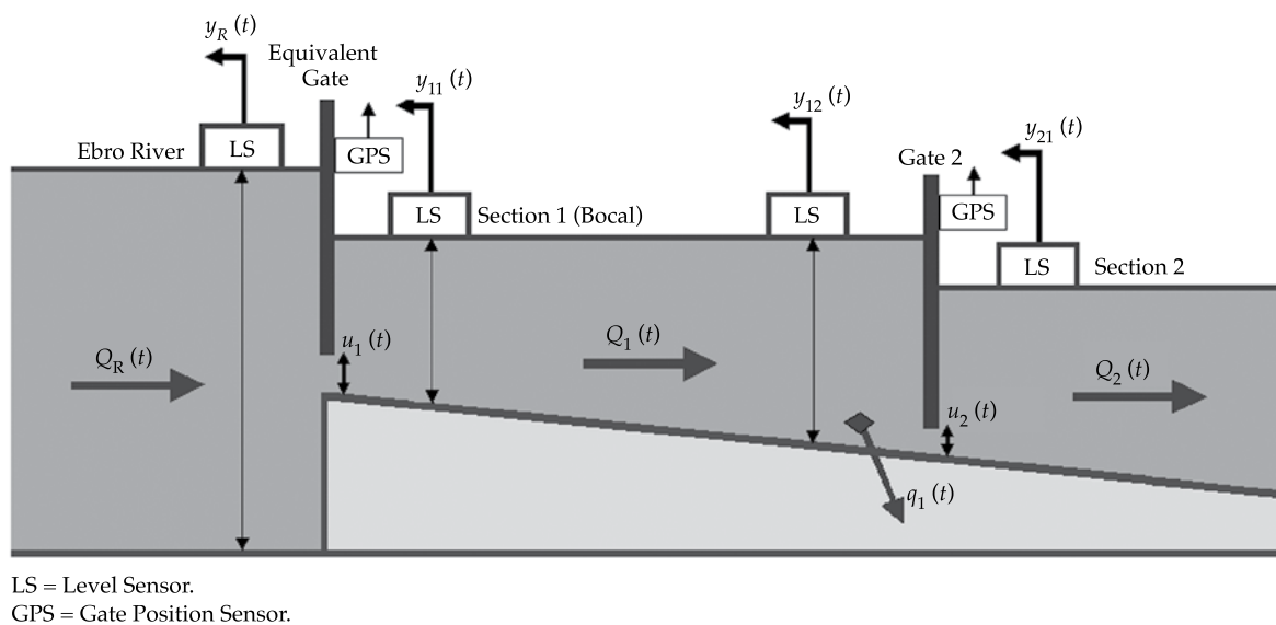
Figure 1. Diagram of Section 1 (Bocal) of the main Imperial de Aragón Canal.
