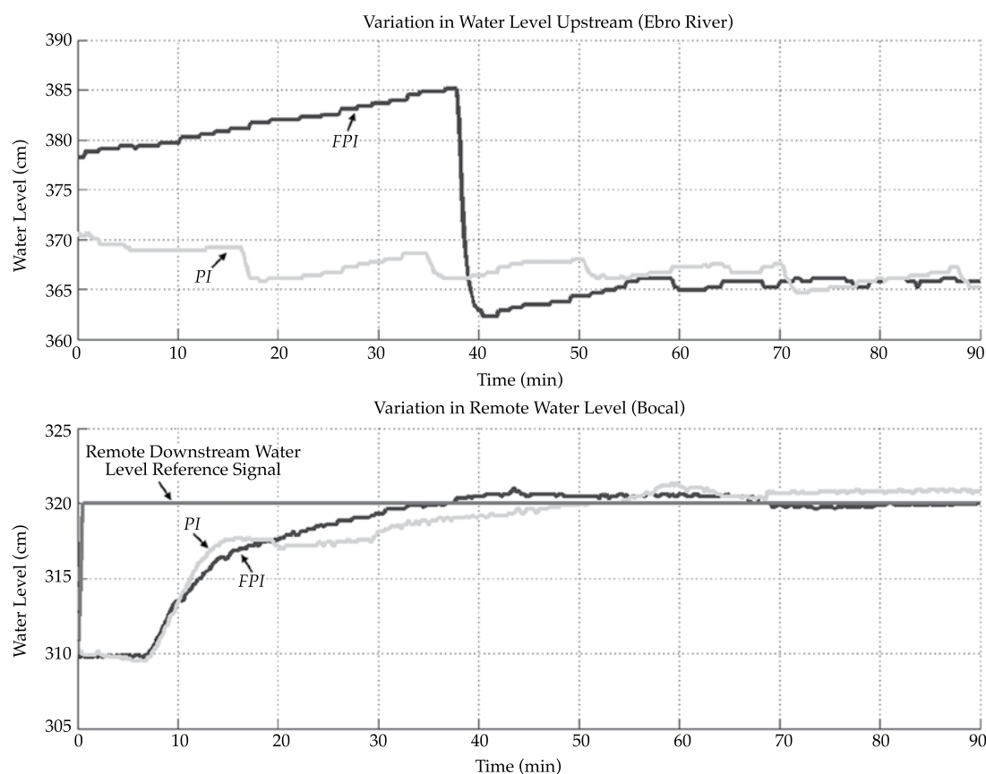
Figure 10. Comparative Experimental Results from the Real-time Functioning of the Water Distribution Control System in the Bocal with FPI and PI Controllers when Discharge Increases.
