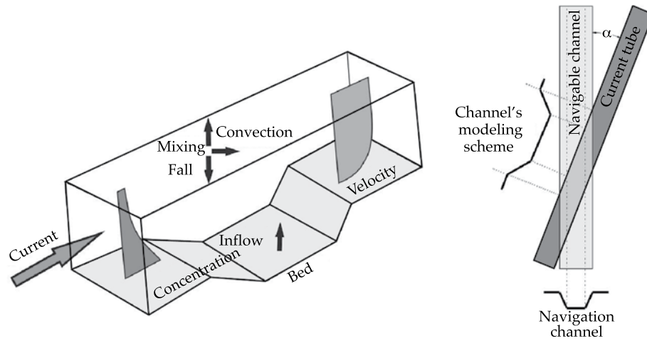
Figure 2. Control Volume for the 2D-V Model.
