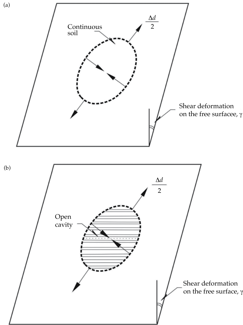
Figure 5. Free-field shear distortion in a medium without and with excavation.
