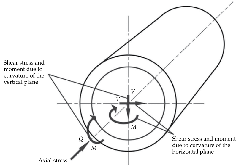
Figure 6. Longitudinal forces and moments caused by waves propagated along the tunnel axis.
