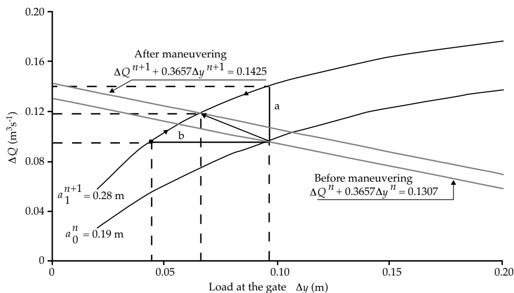
Figure 4. Run of the flow and water depth to maneuver the gate according to change in demand.
