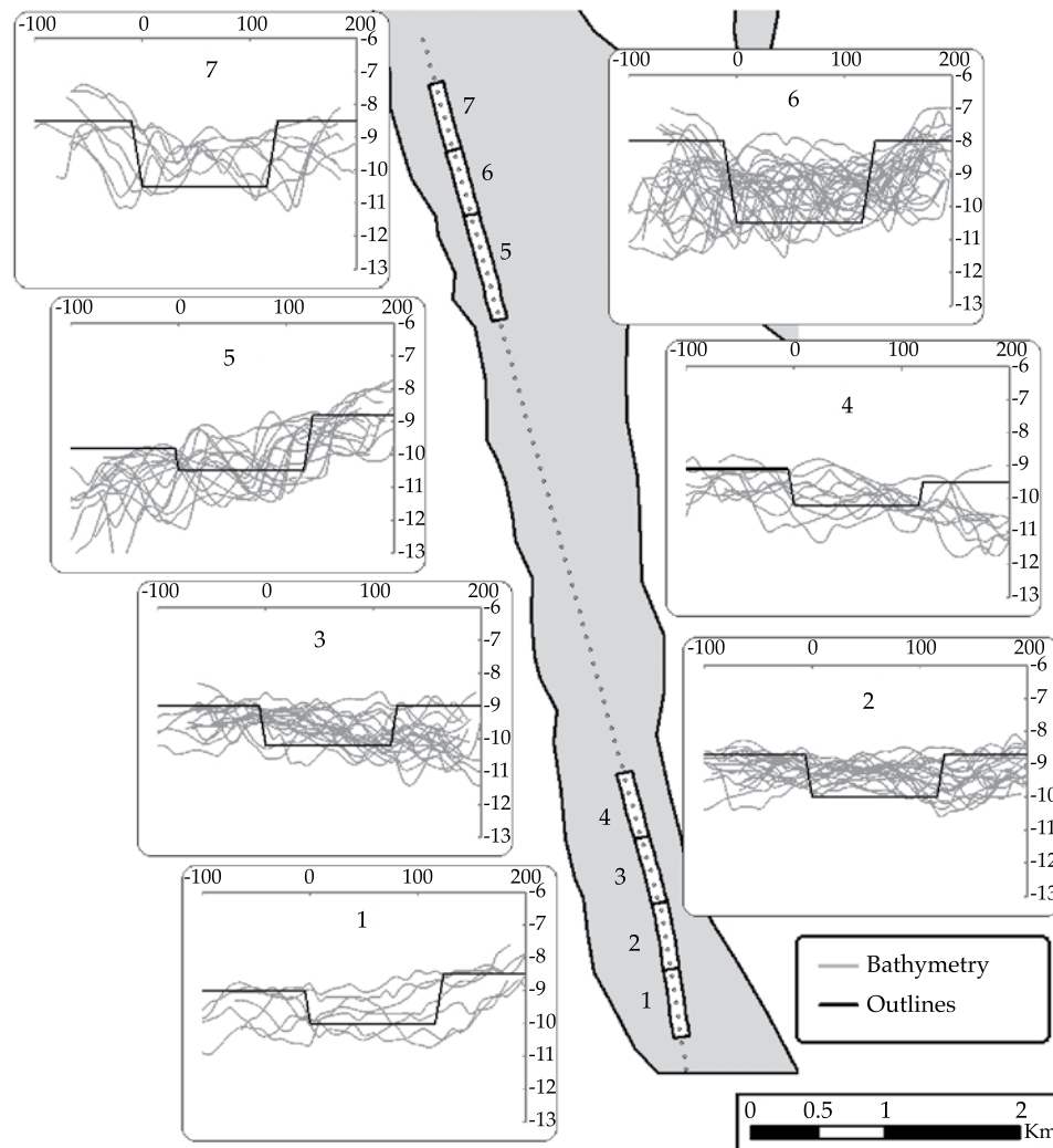
Figure 8. Outline of the dredged cross sections of the sub-sections.
