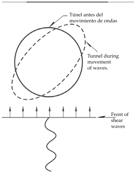
Figure 2. Ovaling deformation in a circular cross-section of the tunnel.
