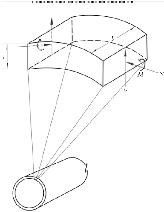
Figure 8. Circumferential stresses and moments caused by waves propagated perpendicular to the tunnel axis.
