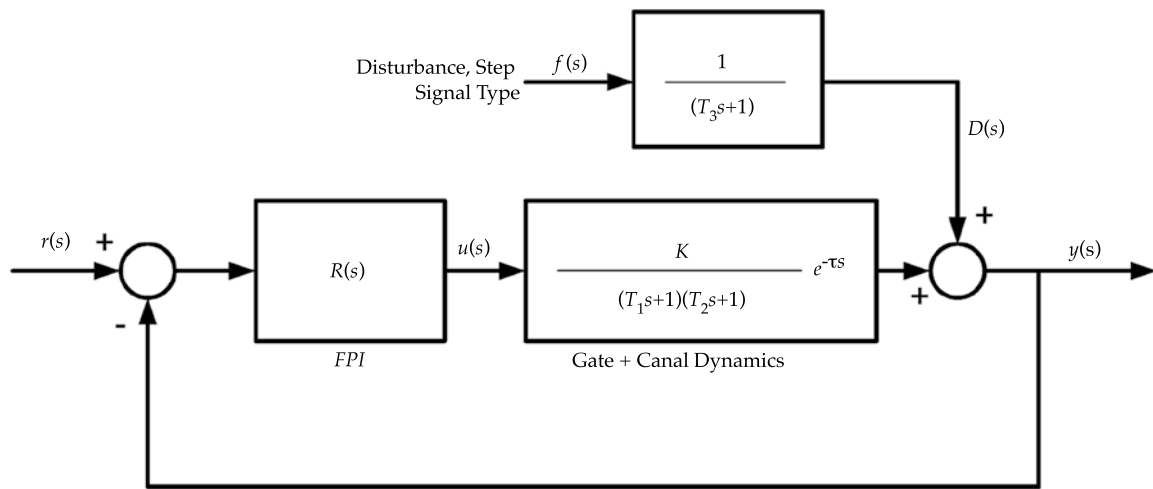
Figure 5. Block Diagram for the Fractional Order Control System for water Distribution in the Bocal
