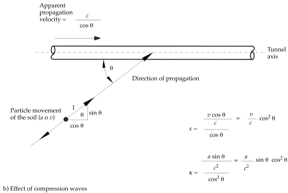
Figure 4. Deformations in the soil resulting from the oblique incidence of flat waves S and P.
