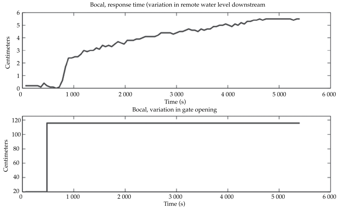
Figure 3. Time Response of the Bocal with a step signal for the gates upstream.
