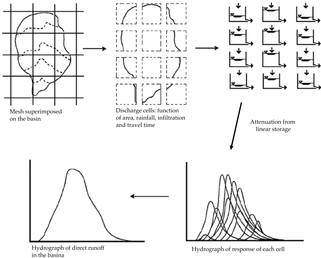
Figure 3. Conceptual Model of the Clark Method for Distributed Parameters (adapted from Kull and Feldman, 1998).
