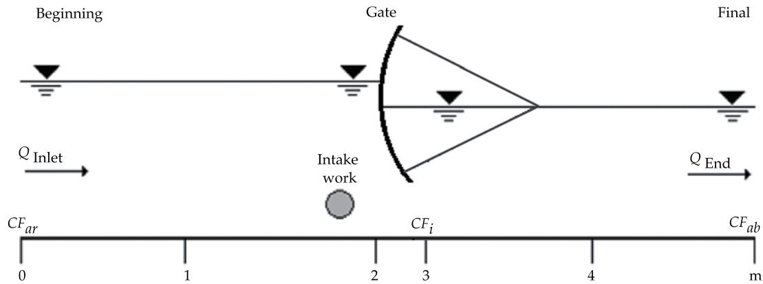
Figure 1. Discretization of a section of the irrigation canal.
