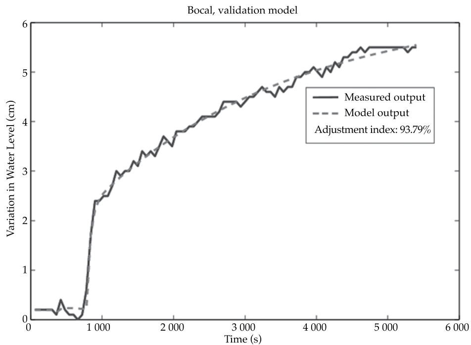
Figure 4. Results from Validating the Nominal Mathematical Model for the Water Distribution in the Bocal.
