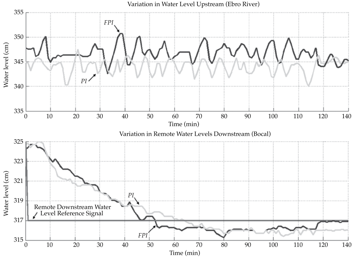
Figure 9. Comparative Experimental Results for the Real-time Functioning of the Water Distribution Control System in the Bocal with FPI and PI Controllers when Discharge Decreases.
