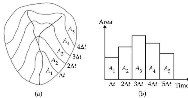
Figure 2. (a) Isochrones and (b) time-area histogram for a basin (adapted from Saghaian et al. 2002).
