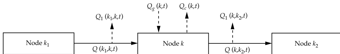
Figure 4. Balance of natural variables at general node k .
