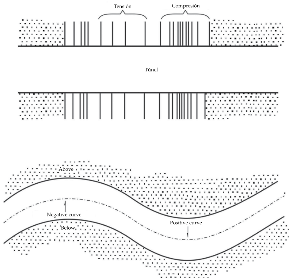
Figure 1. Axial and flexural deformations along the tunnel axis.
