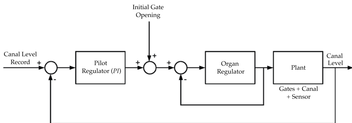
Figure 8. Functional Block Diagram for the Water Distribution Control System in the Bocal.
