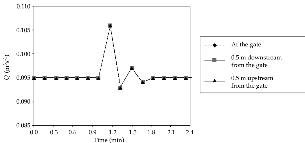
Figure 5. Progressive maneuvering with resetting the water depth and constant flow.
